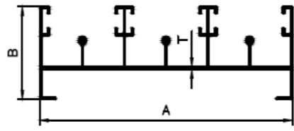
3 TRACK BOTTOM
