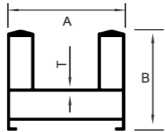
2 TRACK
