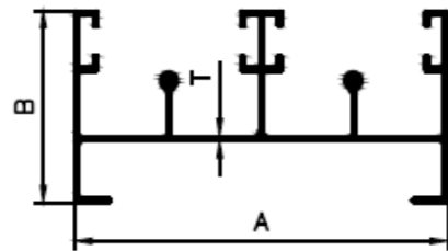
2 TRACK BOTTOM
