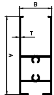
BEARING BOTTOM
