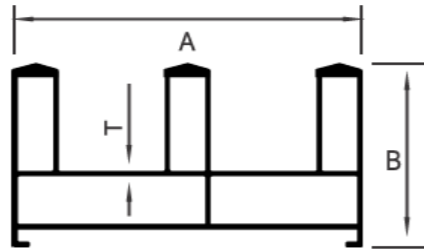
3 TRACK
